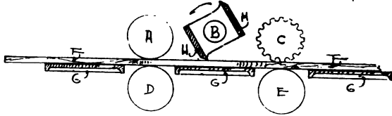
A-Delivery Roller. D-Roller. G-Work Table. B-Cutter Head. E-Roller. M-Knives. C-Feed Roller. F-Board.
