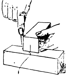
Center Lines FIG. 143.
