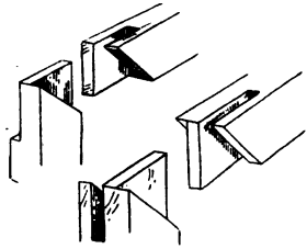
Stretcher Joint.
